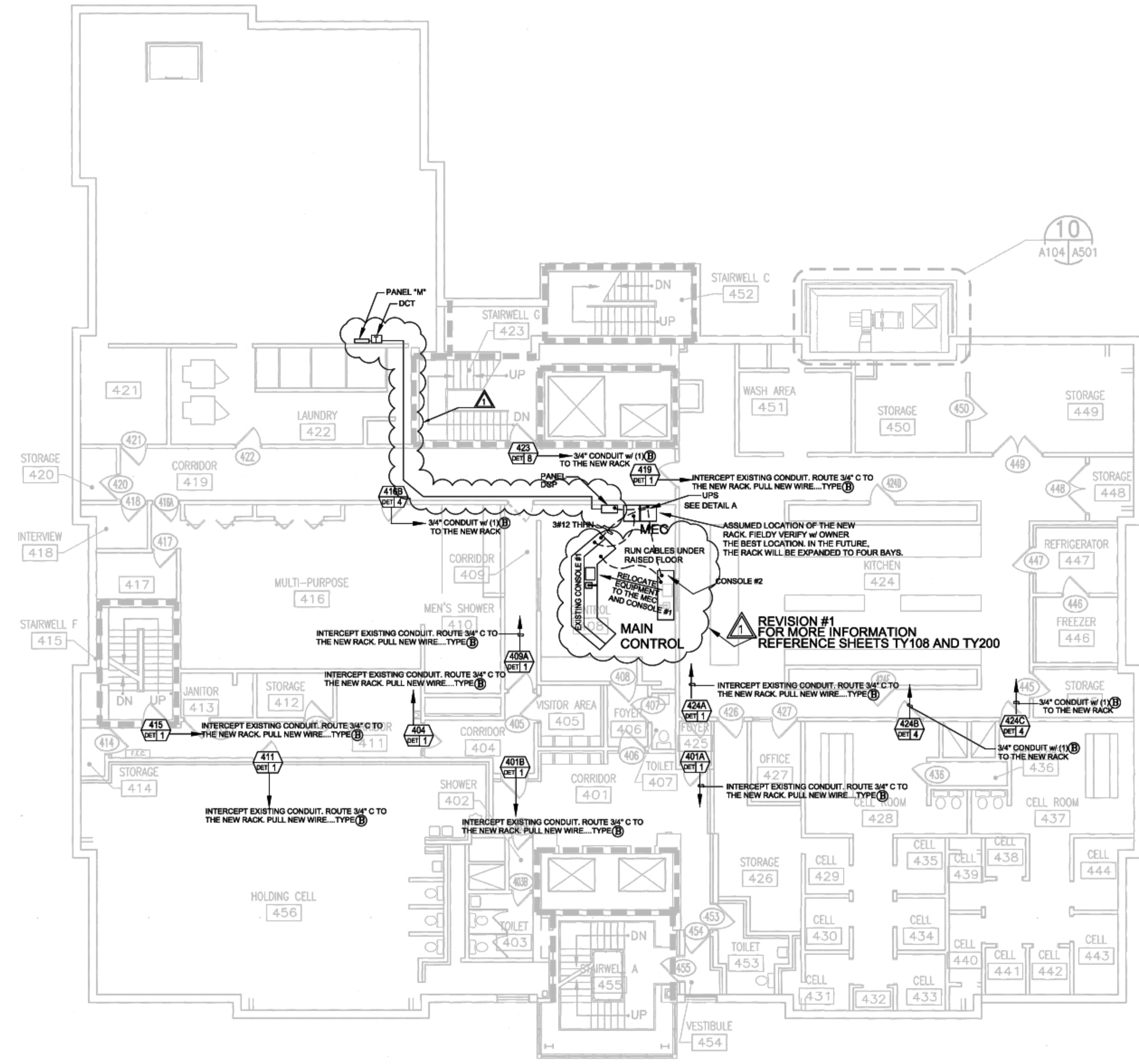
FOURTH FLOOR NEW WORK PLAN SCALE: 1/8" = 1'-0"
